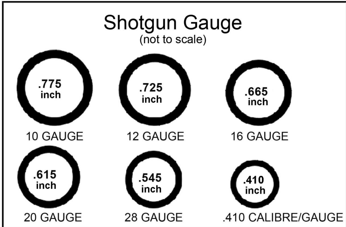
Figure 29. Shotgun Gauges
